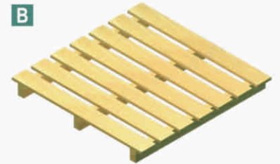
TWO WAY SINGLE DECK WING TYPE
